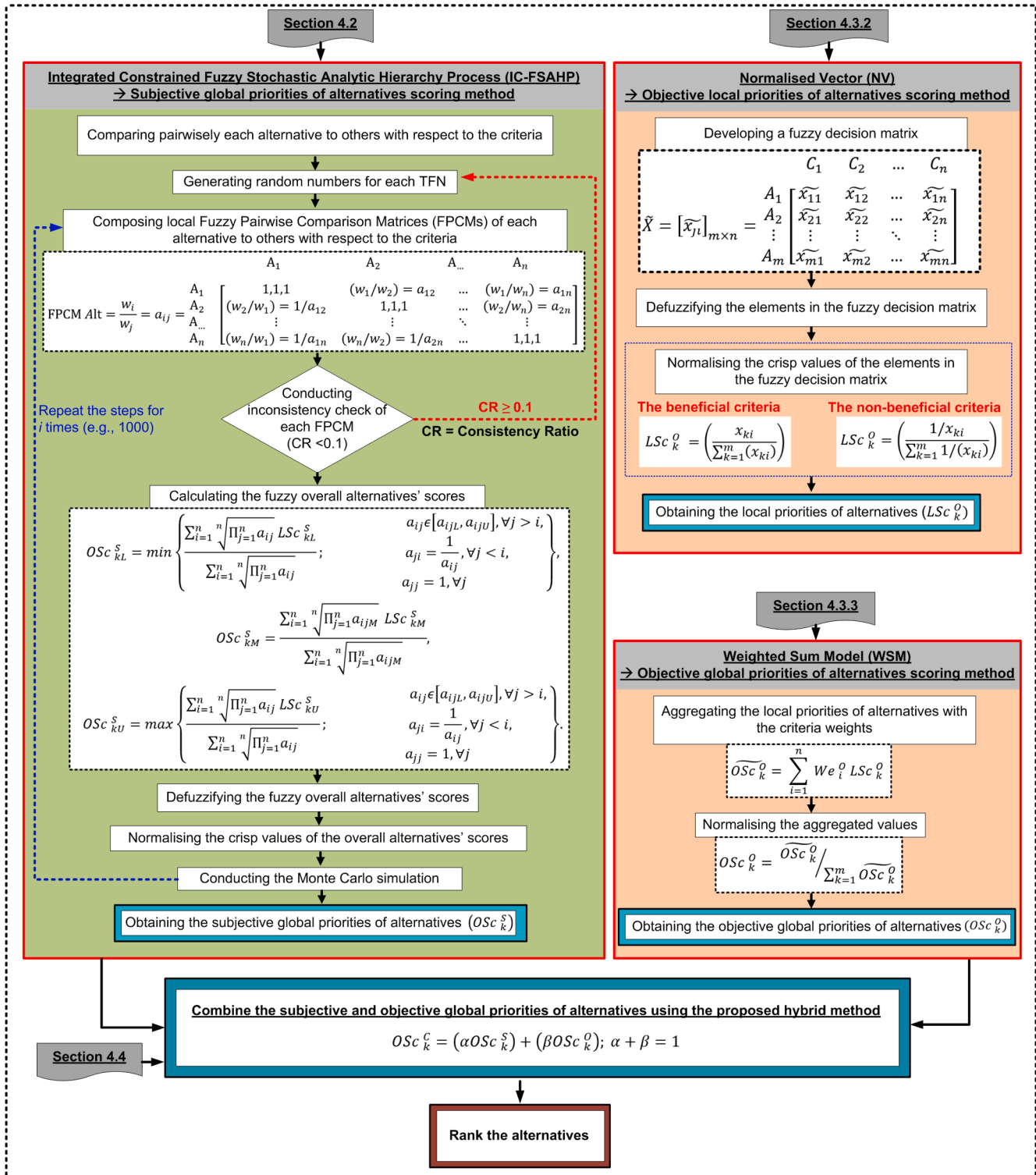
Fig. 7. Flowchart of proposed novel hybrid MCDM method for scoring the alternatives.
