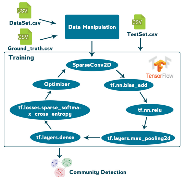
Fig. 2. CNN workflow with TensorFlow.
