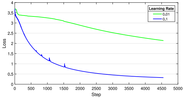
Fig. 7. CNN Gradient descent optimizer with 6 Kernels 3 \times 3 .
