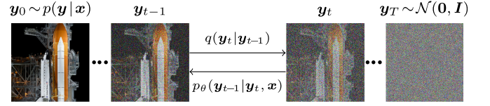
Fig. 2. The forward diffusion process q (left to right) gradually adds Gaussian noise to the target image. The reverse process p (right to left) iteratively denoises the target image, conditioned on a source image \mathbf{x} . (Source \mathbf{x} is not shown.).
