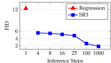
Fig. 12. FID score versus number of inference steps for 64 \times 64 \rightarrow 256 \times 256 super-resolution. Regression (red) requires one step. All SR3 results (blue) are generated from the same denoising model but different inference noise schedules.
