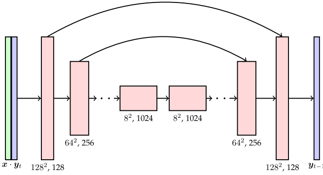
Fig. 3. Depiction of U-Net architecture of SR3. The low resolution input image x is up-sampled to the target resolution using bicubic interpolation, and concatenated with the noisy high resolution output image y_t . We show the activation dimensions for a 16 \times 16 \rightarrow 128 \times 128 super resolution model. We perform self-attention on 16 \times 16 feature maps.
