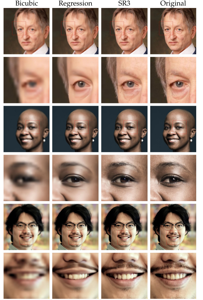
Fig. 6. Results of a SR3 model ( 64 \times 64 \rightarrow 512 \times 512 ), trained on FFHQ, and applied to images outside of the training set.
