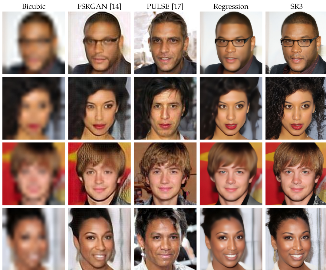
Fig. 8. Comparison on 4× face super-resolution ( 16 \times 16 \rightarrow 128 \times 128 ). Reference images are removed for privacy concerns.
