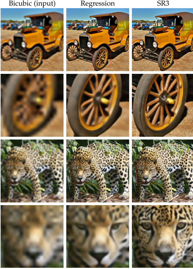
Fig. 4. Super-resolution results ( 64 \times 64 \rightarrow 256 \times 256 ) for SR3 and Regression on ImageNet test images. Both models use the same architecture and training data. We display the full image and an enlarged patch to show fine-grained details.
