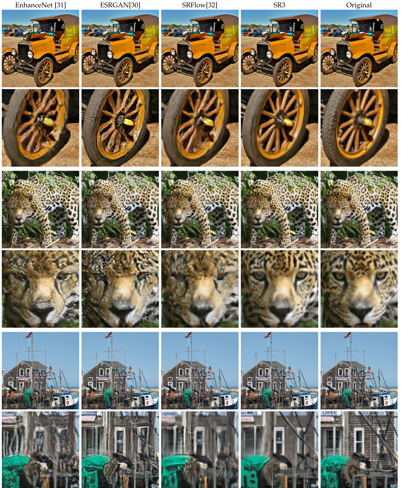
Fig. 7. SR3 and state-of-the-art methods on 4\times super-resolution ( 64\times 64 \rightarrow 256\times 256 ) applied to ImageNet test images. The outputs of EnhanceNet and ESRGAN are sharp, but include artifacts especially when inspecting enlarged patches. We found that ESRGAN trained on ImageNet-1 M produced similar artifacts. SR3 outputs seem to resemble the original images the most, but one can still find patches in the original images that contain more interesting texture than in SR3 outputs.
