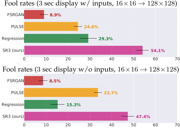
Fig. 9. Face super-resolution human fool rates (higher is better, for photo-realistic samples one would expect a fool rate close to 50%). Outputs of four models are compared to ground truth. (top) Task-1, subjects are shown low-resolution inputs. (bottom) Task-2, inputs are not shown.
