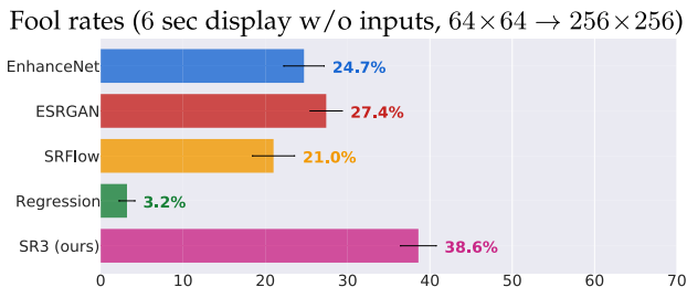
Fig. 10. ImageNet super-resolution fool rates. Model outputs are compared to ground truth with pair of images shown for 6 seconds.
