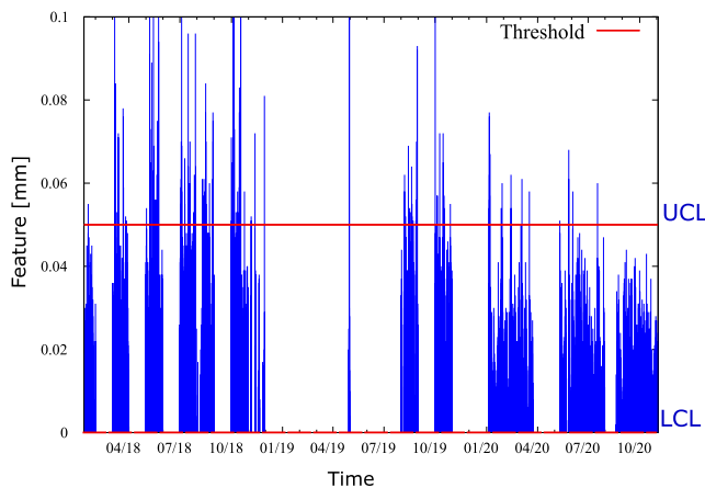
Fig. 8. Measurements of a single feature captured for all monitored machines during the period 2018–2020. For this feature, the upper limit tolerance is indicated with a horizontal red line, and the target value is zero. (For interpretation of the references to colour in this figure legend, the reader is referred to the web version of this article.)
