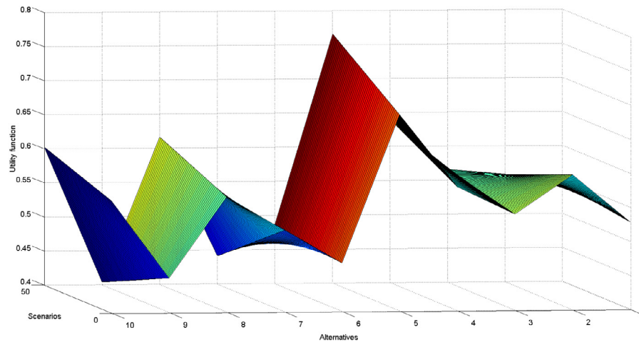
Fig. 7. Influence of change of criterion weights on change of utility functions.
