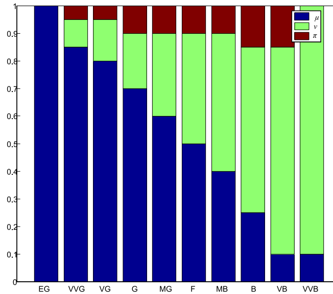
Fig. 2. Plots of IFNs [\mu, \nu, \pi] .
