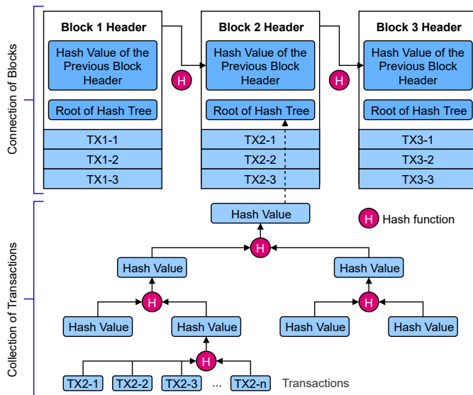
Fig. 1. General structure of a blockchain, in which blocks connected with each other through their respective hash codes.
