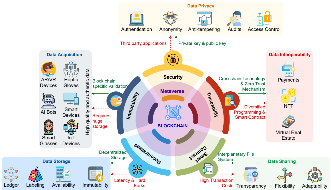
Fig. 3. Blockchain for technical aspects in the metaverse.
