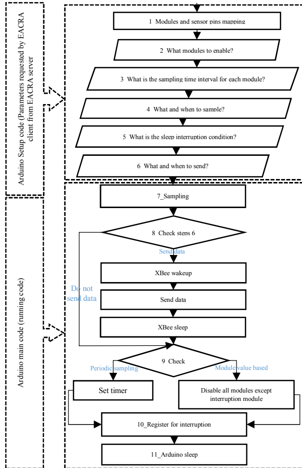
Figure 11 EACRA Client algorithm.
