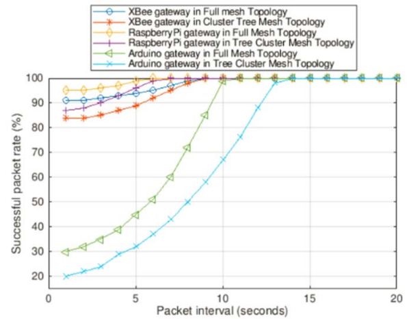
Figure 5 Successful packet rate in different packet time interval of the three gateways in different network topologies.
