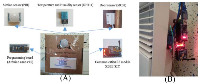
Figure 2 WSN Sensor and actuator.
