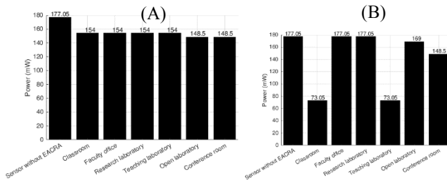
Figure 12 Energy optimization, during the day (A) and night (B) using the EACRA algorithm.
