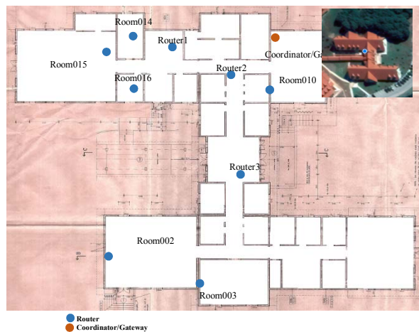
Figure 3 The Network test architecture in ground floor of building 7.
