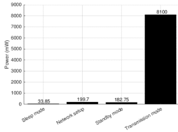
Figure 7 XBee RF power consumption in different modes.
