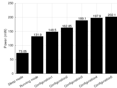
Figure 6 WSN node energy consumption of different configurations.
