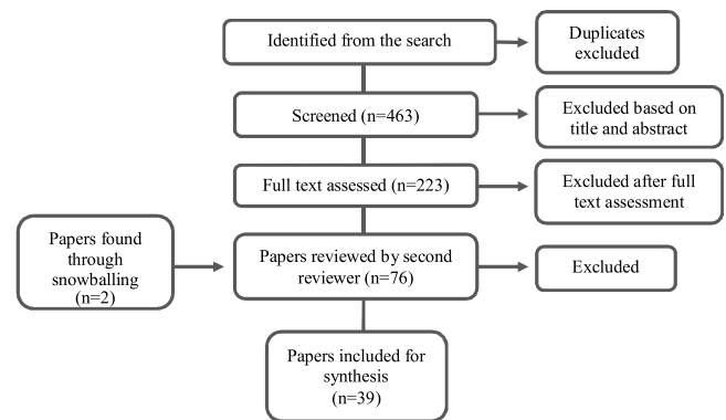
Fig. 3. Inclusion flowchart.
