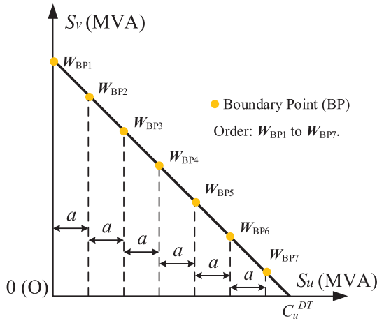
Fig. 3. The generation of all boundary points. W_{BP1}-W_{BP7} are one-by-one generated.
