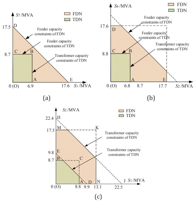
Fig. 13. (a) 2D dispatchable region projections of TDN and FDN of single-loop feeder pairs of 7-feeder IEEE RBTS case (F1, F7); (b) 2D T dispatchable region projections of TDN and FDN of multi-connected feeder pair of 7-feeder IEEE RBTS case (F2, F6); (c) 2D dispatchable region projections of TDN and FDN of feeder pair from the same substation transformer of 7-feeders IEEE RBTS case (F1, F2).
