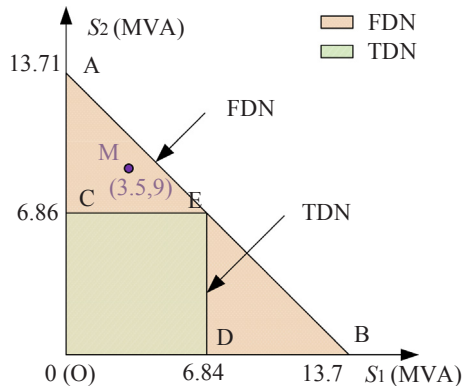
Fig. 7. Dispatchable region projections of FDN and TDN of single-loop network case (simplified).
