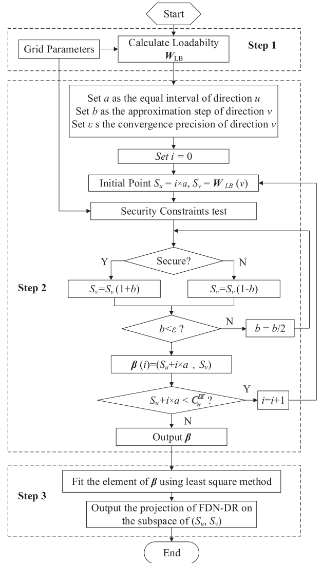
Fig. 2. The flow chart of the proposed simulation-based observation approach of the dispatchable region of FDN.
