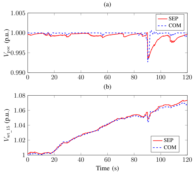
Fig. 8. Voltages at POC and WT15 for Case 1.
