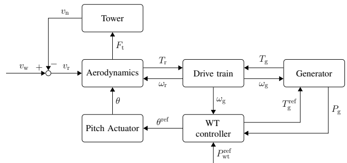
Fig. 3. Single wind turbine system [15].
