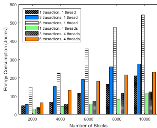
Figure 9: Energy consumption of the chain verification process
