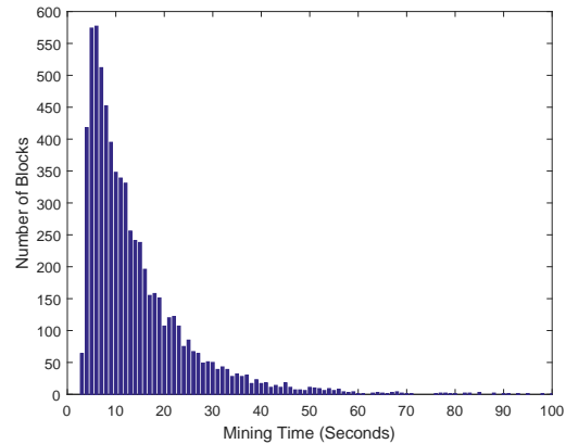
Figure 7: The distribution of mining time v.s. number of blocks.
