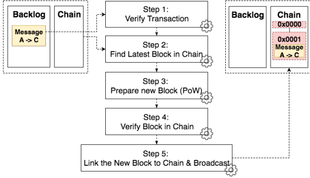
Figure 2: The mining process in the MobiChain system
