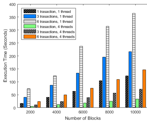
Figure 8: Execution time of the chain verification process.
