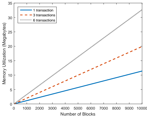
Figure 6: The memory utilization when the number of blocks increases.
