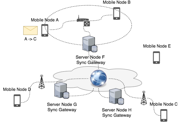
Figure 1: The MobiChain system model.
