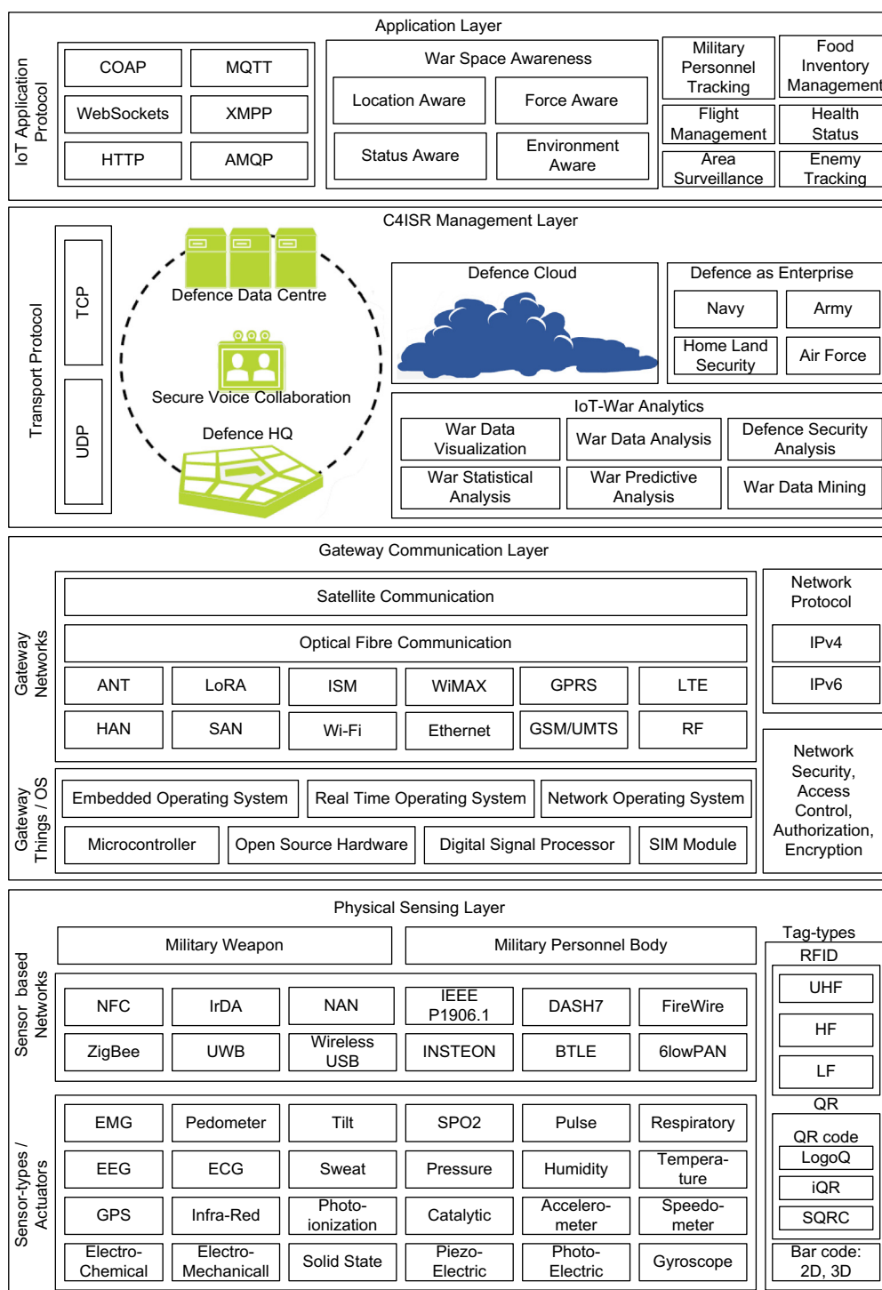
Figure 12 IoTNetWar architectural framework.
