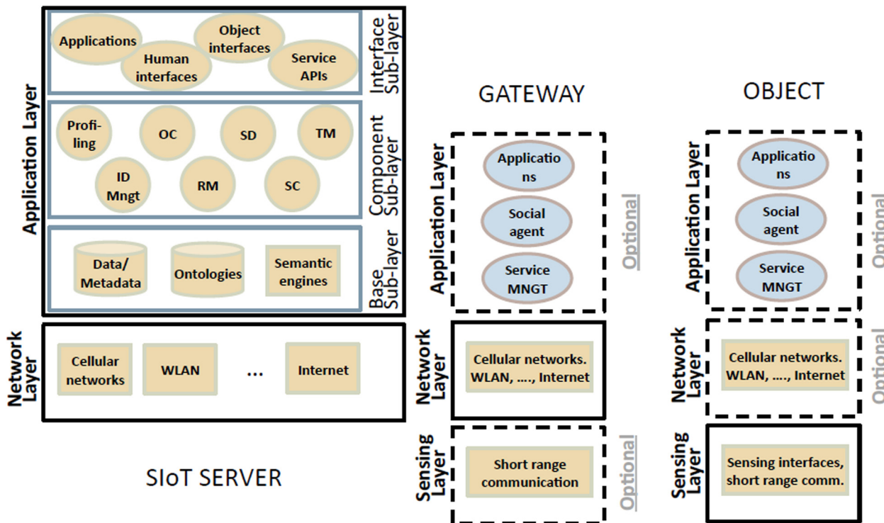
Figure 9 Social IoT architecture, following the three layer model made of the sensing, network, and application layer.
