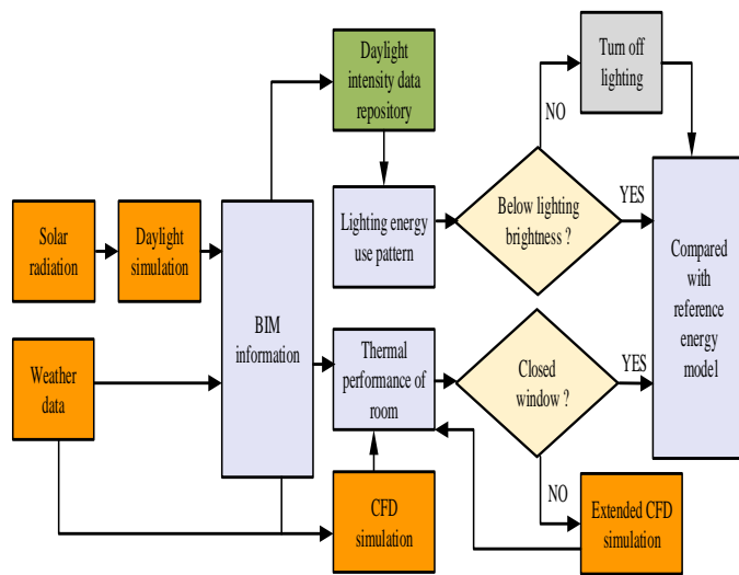
FIGURE 5. Conceptual framework of the smart BEMS [45].
