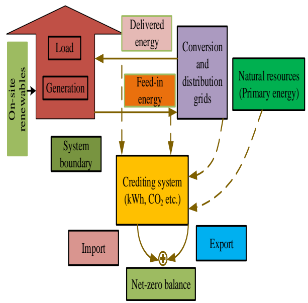
FIGURE 2. Schematic of a typical nZEB
