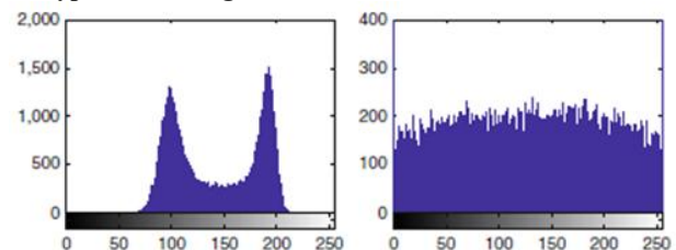
a)Histogram of original finger print image
