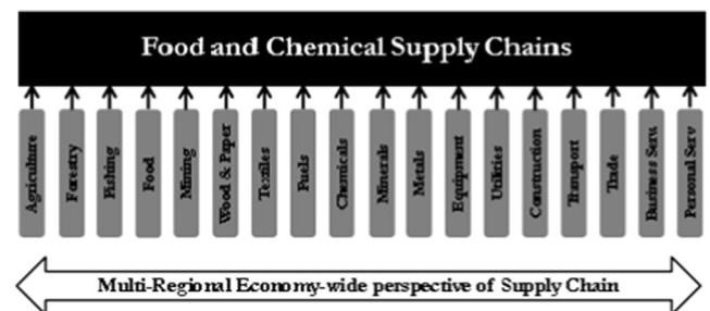
Fig. 2. Whole economy representation based on an EIO framework.
