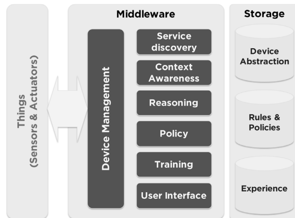
Fig. 4. Typical SOA for intelligent SH system.
