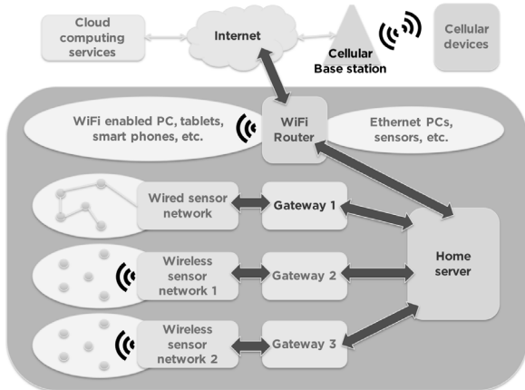
Fig. 2. Typical heterogeneous home network.
