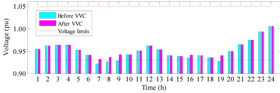
Fig. 7. Voltage behavior in bus 10 before and after the VVC.
