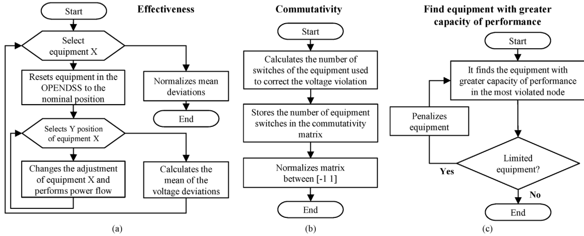
Fig. 5. Flow graphs to obtain the matrices. (a) Effectiveness. (b) Commutativity. (c) Equipment with greater capacity of performance.
