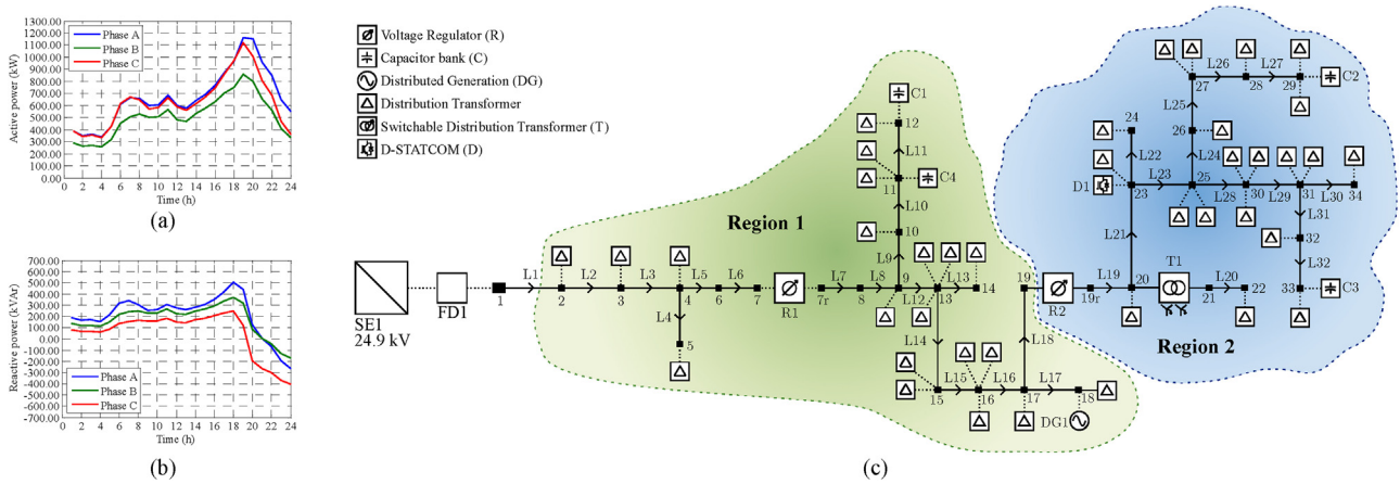
Fig. 9. Modified IEEE 34 node test feeder. (a) Active and (b) reactive power curves in the substation. (c) Network topology.
