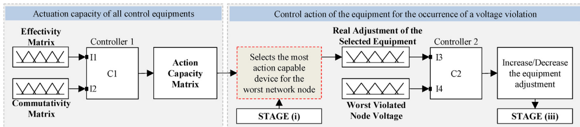
Fig. 4. Flowchart of Stage (ii). Set of fuzzy controllers to the proposed application.
