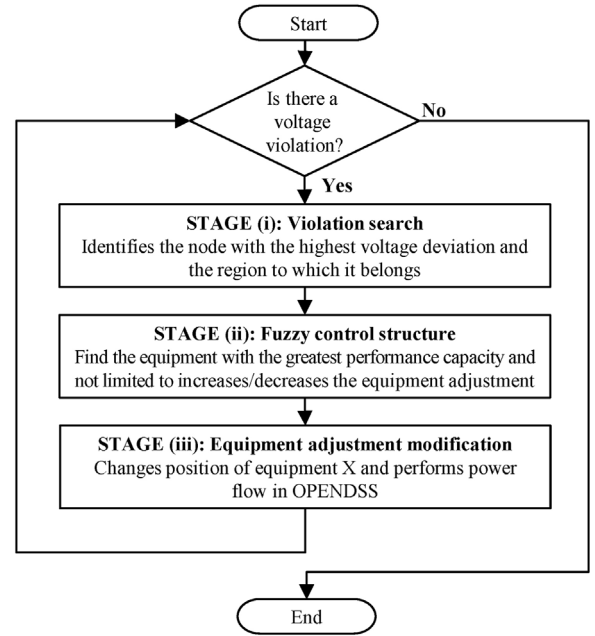
Fig. 3. Main stages of the coordinated VVC algorithm.
