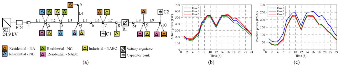
Fig. 6. Distribution test network. (a) Network topology. (b) Active power behavior. (c) Reactive power behavior in substation.
