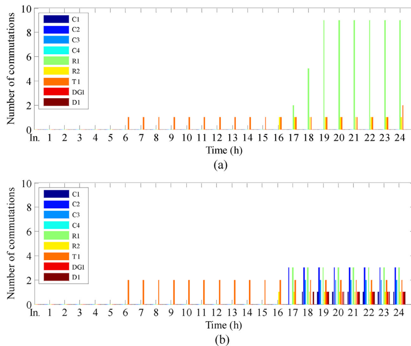
Fig. 12. Behavior of the equipments commutation along 24 h with (a) EM enabled and CM disabled and with (b) ME and CM enabled.
