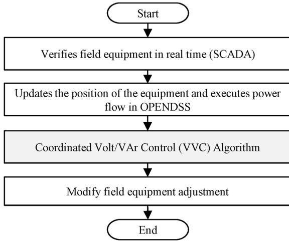
Fig. 2. Architecture of the proposed to the coordinated VVC.
