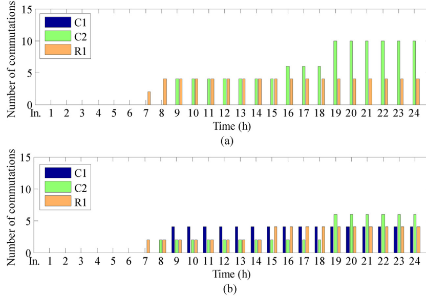
Fig. 8. Evolution of commutations in the system with (a) EM enabled and CM disabled and with (b) EM and CM enabled.
