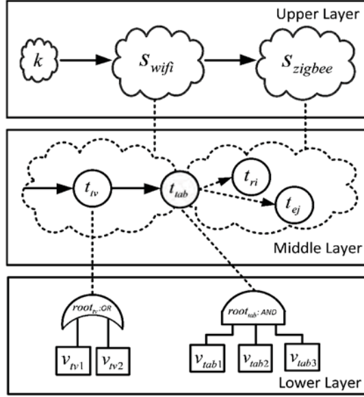
Figure 3: The attack paths in the smart home.
