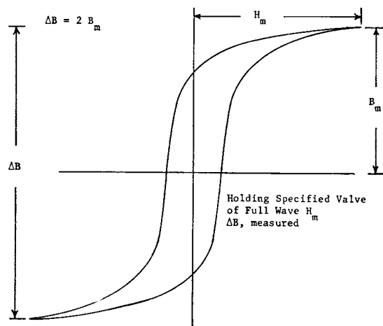
FIG. X3.2 Sine-Current SCM Flux-Current Loop for Test Described in 10.2
