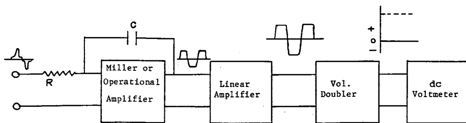
FIG. X1.2 Miller Integrator
