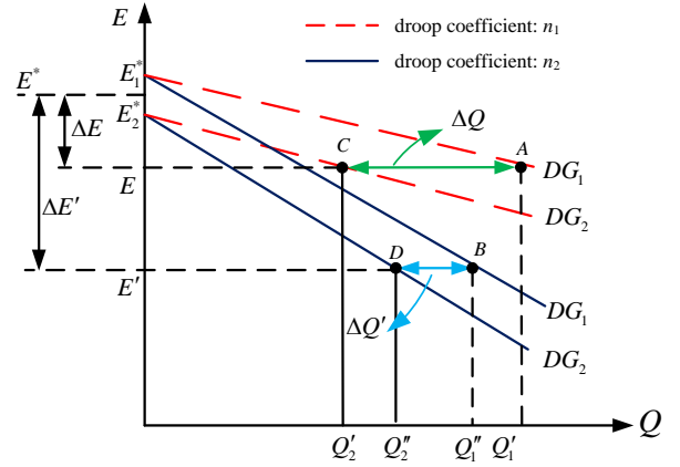
Fig. 3. Characteristic curves of the reactive power droop control with two DGs [104].
