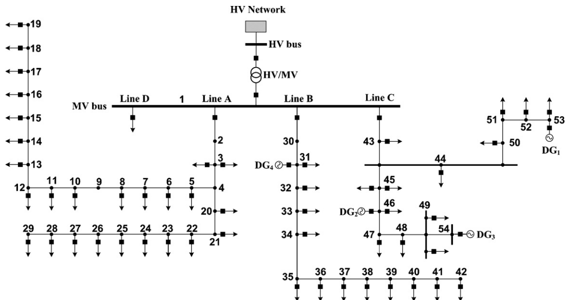
Fig. 3. Italian radial network for test case.
