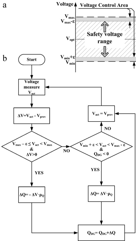
Fig. 1. (a) Control ranges; (b) flow chart of the sensitivity method.
