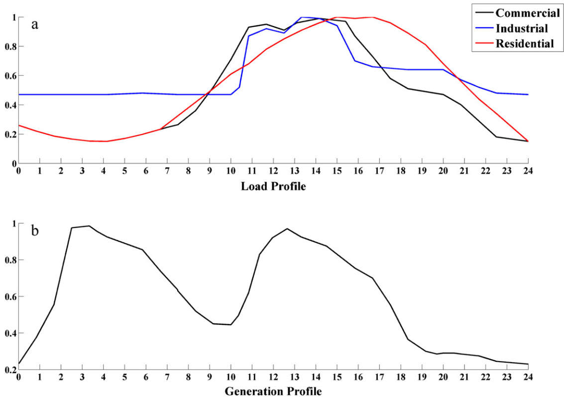
Fig. 5. (a) Load demand profiles; (b) power generation profile.
