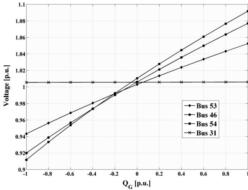
Fig. 4. Bus voltage as a function of reactive power injections at the same bus.
