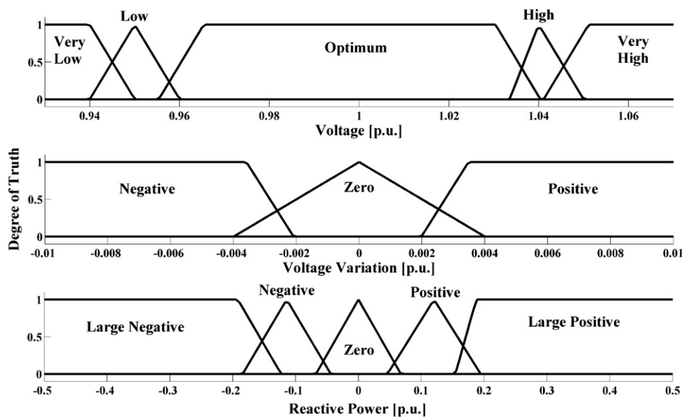
Fig. 2. Membership functions of the fuzzy controller.
