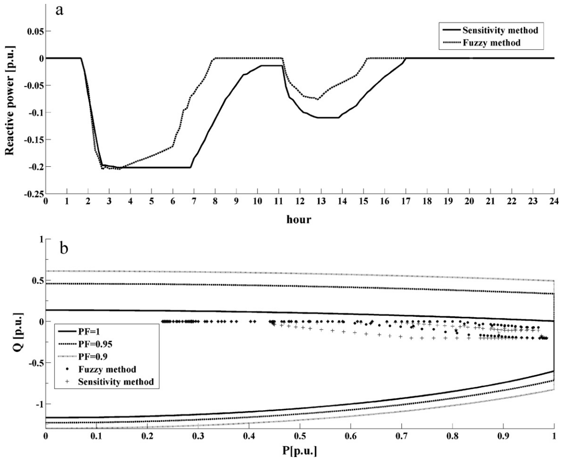
Fig. 7. (a) Reactive power at bus 54; (b) capability coverage with capability curve.
