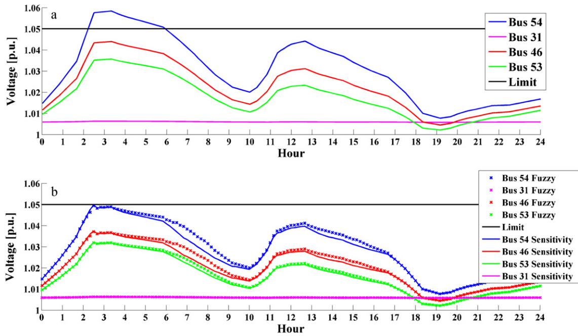
Fig. 6. (a) Voltage profiles without voltage regulation at DWT buses; (b) voltage profiles with voltage regulation at DWT buses.
