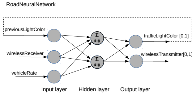
Figure 9: Adaptive Agent's Neural Controller.
