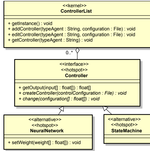
Figure 5: Class diagram of FIoT - Controllers.
