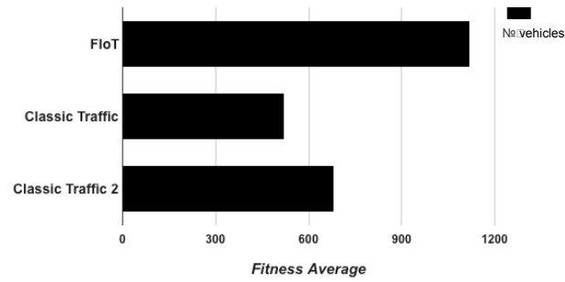
Figure 12: Comparison of the FIoT approach and conventional systems in the first scenario.
