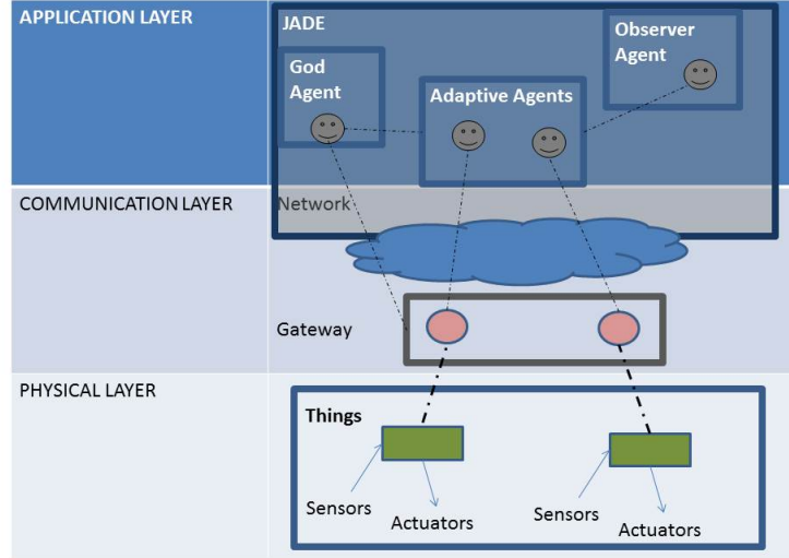
Figure 1: An agent-based model to generate IoT applications.
