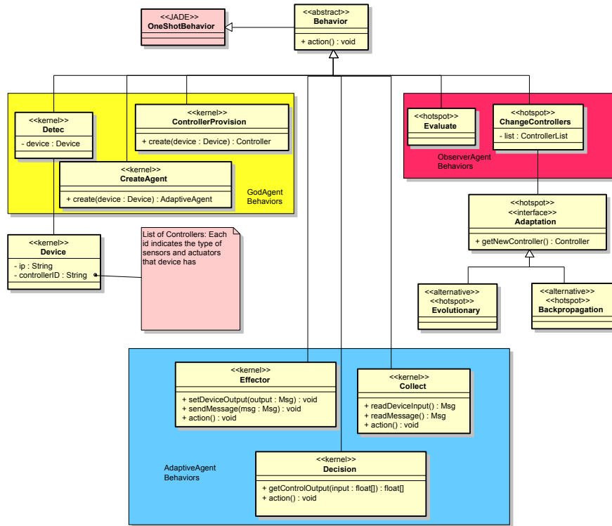
Figure 4: Class diagram of FIoT - Behaviors.
