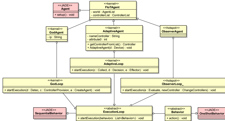
Figure 3: Class diagram of FIoT - Agents.
