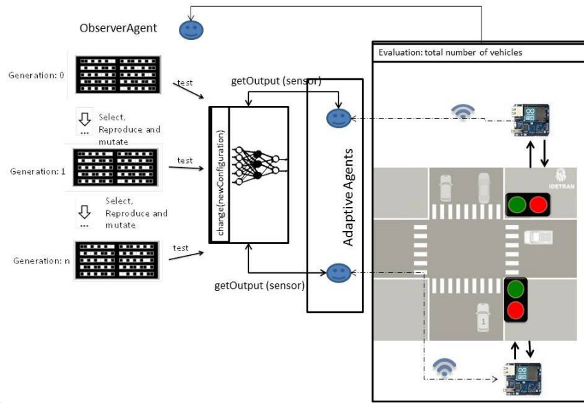
Figure 10: Performing an adaptive process to adjust the Traffic Neural Controller weights. Figure adapted from [41]. P.7.
