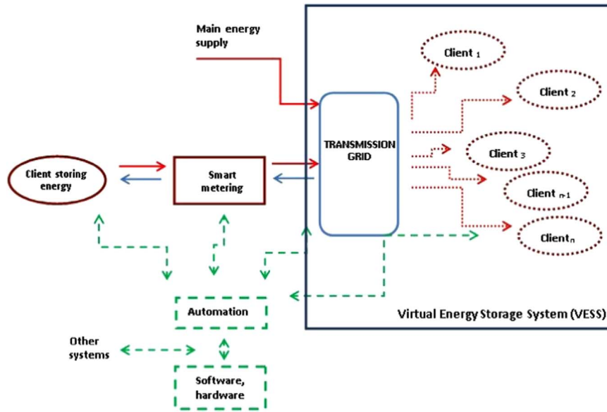
Fig. 3. Virtual Energy Storage System (VESS).
