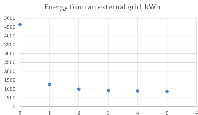
Fig. 6. Energy received from the grid by use of different amount of batteries 24 kW h 0–5 batteries).
