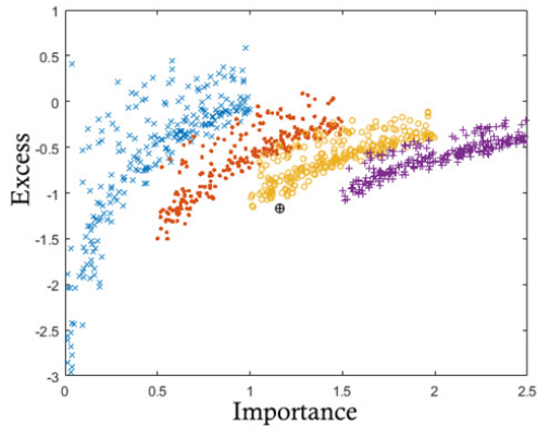
Fig. 3. Scatter graph showing examples of importance values selected randomly from a Gaussian distribution with means 0.5 (x), 1 (•), 1.5 (◊) and 2 (+) and variance 1. Each symbol represents a node in the 100-node randomly connected network, plotted according to its power deficit (or negative excess) and the importance weight it was given. One fifth of nodes in the network are given mean capacity \bar{\Lambda} = 1 , and the remaining consumers \bar{\Lambda} = -1 , all variances are fixed at \sigma = 0.5 .
